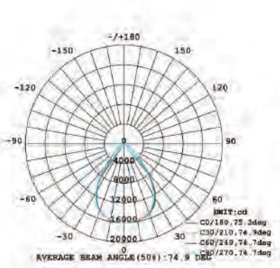
19" 60° PC Reflector
