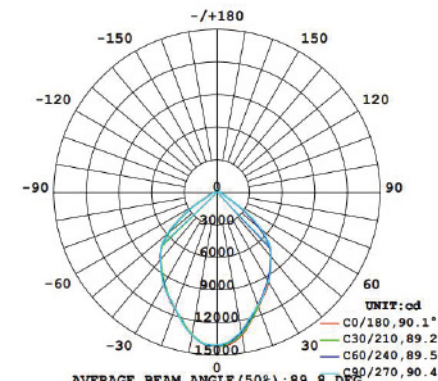
19" 90° PC Reflector
