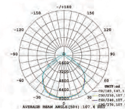
120° PC Reflector
