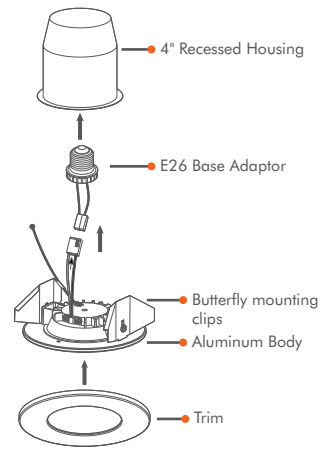
4" Recessed Housing
