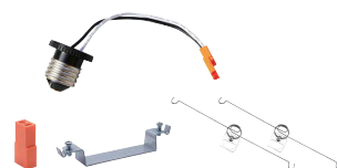
E26 adapter and Mounting Brackets for 5" & 6" housing (sold separately)
