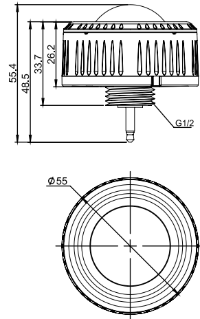
FDUFO-PRO-PIR-Sensor SKU#101377
